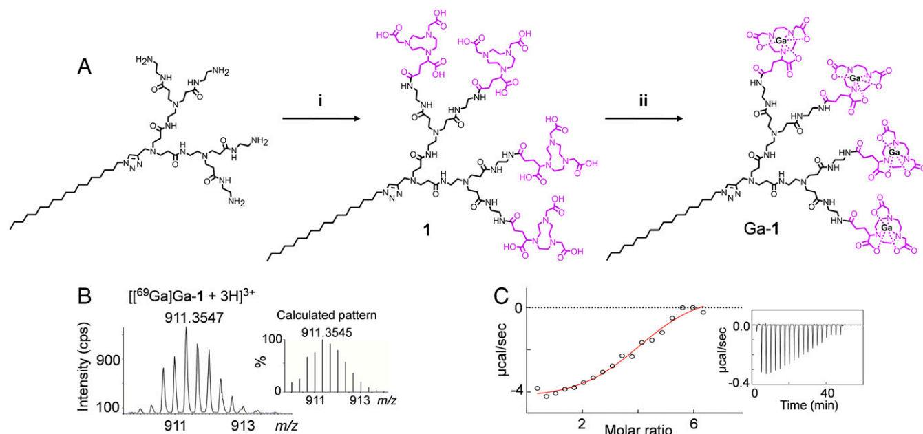
Fig. 2. Synthesis of the amphiphilic dendrimer 1 and its chelation with the nonradioactive isotope ^{69}\text{GaGa}^{3+} at the terminals. (A) Synthesis scheme: (i) (a) NODA-GA(tBu) 3 , PyBOP, NMM, DMF, 30 °C, 72 h; (b)TFA, CH 2 Cl 2 , 30 °C, 16 h. (ii) ^{69}\text{Ga}[\text{GaCl}_3] , 1.0 M HCl, 20 °C, 15 min. (B) High-resolution mass spectrum showing the isotopic pattern characteristic of the triply charged species [[^{69}\text{Ga}]\text{Ga}-1+3\text{H}]^{3+} . The Inset shows the calculated isotopic pattern. (C) Isothermal titration calorimetry (ITC) curve for chelation of \text{Ga}^{3+} with dendrimer 1 . The Inset shows measured heat power versus time elapsed during titration.
